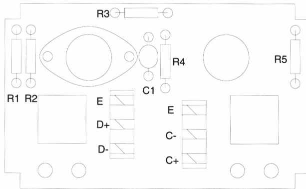
Figure 7.1: The layout of the Acorn terminator PCB
