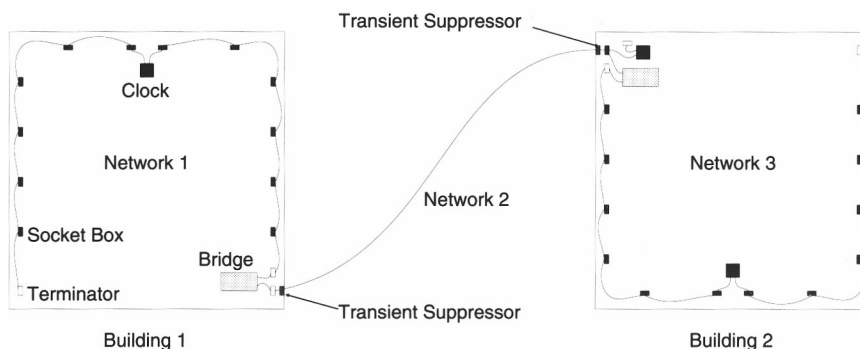
Figure 13.5: External links between buildings
