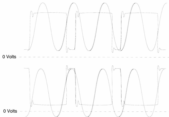
Figure 11.9: External interference on the clock signals
