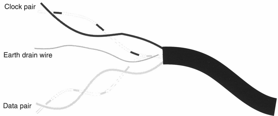
Figure 4.1: Different twist ratios of pairs of wires in Acorn Econet cable
