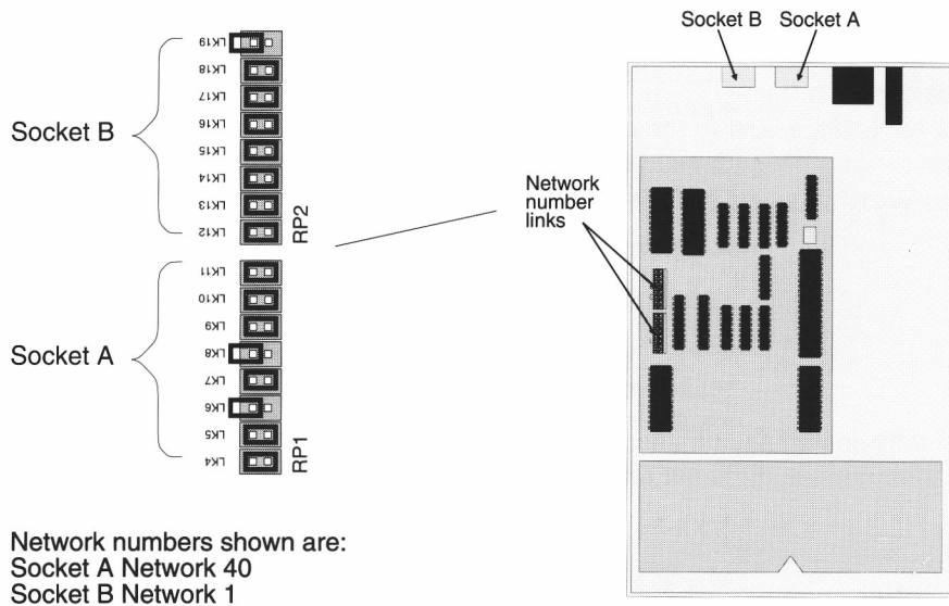
Figure 12.4: Network links on an Acorn Bridge.
