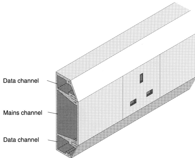
Figure 5.3: Trunking with 2 secondary channels
