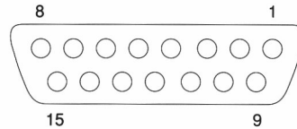
Connections viewed from solder side
