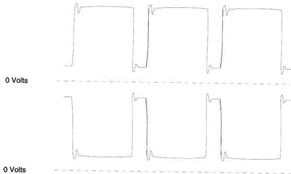
Figure 11.5: Normal clock waveform
