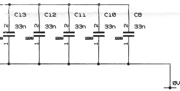
Power Decoupling
