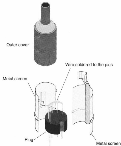
Figure 11.1: Exploded view of a shorting plug.
